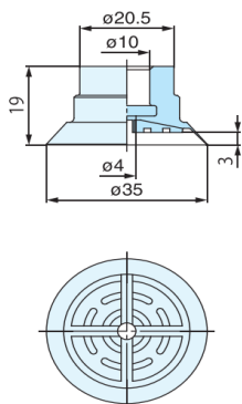
ZP3P-35PTSF [weight:4.7g]
