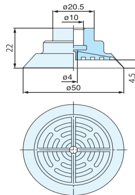
ZP3P-50PTSF [weight:12.4g]
